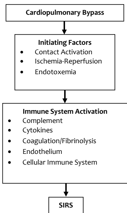
Figure 1: Schematic diagram of the sequence of events by which cardiopulmonary bypass (CPB) may lead to the development of SIRS (systemic inflammatory response syndrome).
