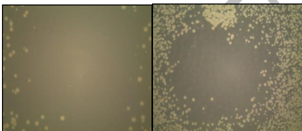
Figure 1. The diameter of the inhibition zone of non-thermal atmospheric argon plasma jet on MRSA at different times of plasma radiation, Left image; after 30 sec, Right image; after 2 minutes
