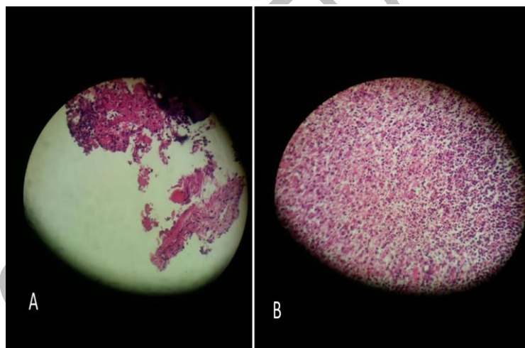
Figure 4. Impact of atmospheric non-thermal plasma after staining with Haematoxylin-Eosin and preparing the pathology sections. A; Pathology image of the control sample, B. Pathology image of the plasma-treated sample.
