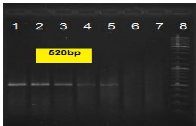
Figure 2. Lanes 1 to 6 including Vibrio Cholerae DNA serial dilution (ng/µl): 10, 5, 2.5, 1.25, 0.625, 0.312; Lane 7: Control; Lane 8: DNA ladder.
