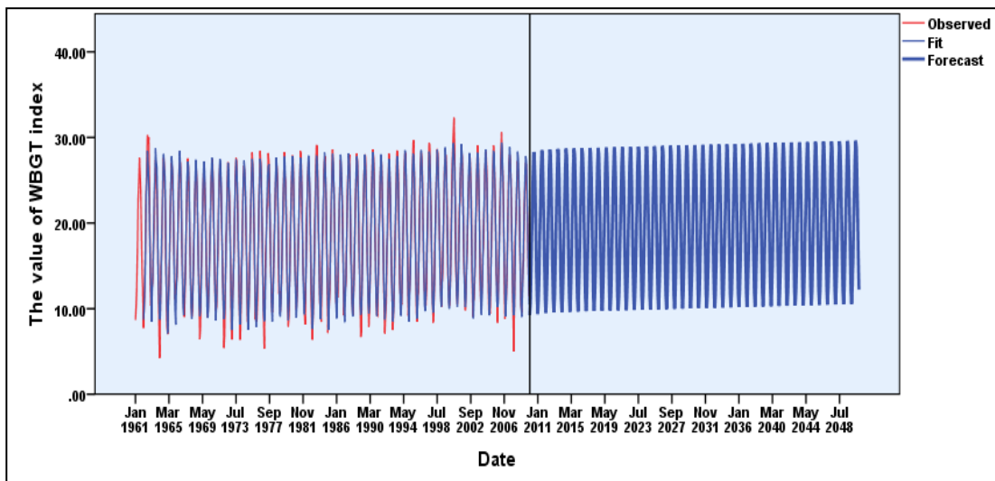
Fig. 2: The fitting of proposed model to observed data and the predicted trend of Tehran's WBGT index.
