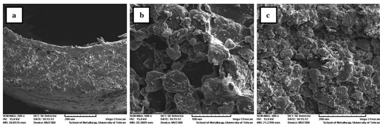
Fig. 2 SEM image of the porous nanocomposite conduit. Cross-section view of conduit (200 \times ) (a), outer layer of conduit wall (500 \times ) (b) and inner layer of conduit wall (300 \times ) (c)
