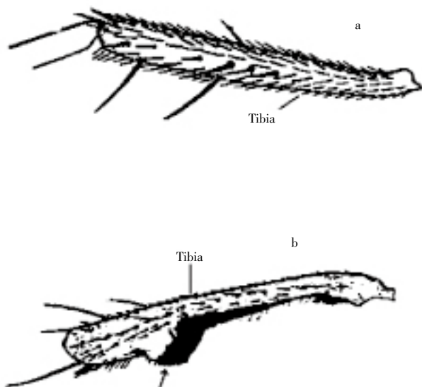
Figure 3. Tibia of mid leg in Fannia . a) F. canicularis without bumps. b) F. scalaris : Tibia with a bulge in the posterior region.
