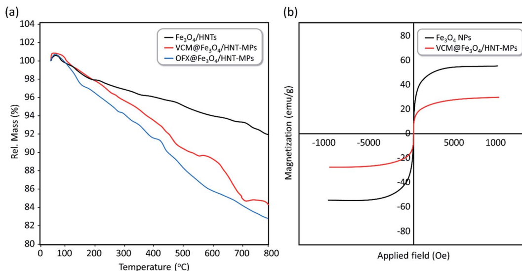
Fig. 3 (a) TGA curves of \text{Fe}_3\text{O}_4/\text{HNTs} , \text{VCM}@Fe_3O_4/\text{HNT}-\text{C}(\text{WR})_3 , and \text{OFX}@Fe_3O_4/\text{HNT}-\text{C}(\text{WR})_3 , composites, under air atmosphere. (b) Room-temperature magnetic-hysteresis curves of \text{Fe}_3\text{O}_4 NPs and \text{VCM}@Fe_3O_4/\text{HNT}-\text{C}(\text{WR})_3 composite.
