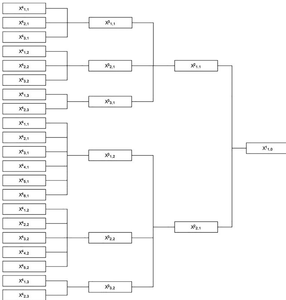
Figure 3. Hierarchical structure of fire, explosion and release of toxic gas of Siri-Assaluyeh pipeline.
