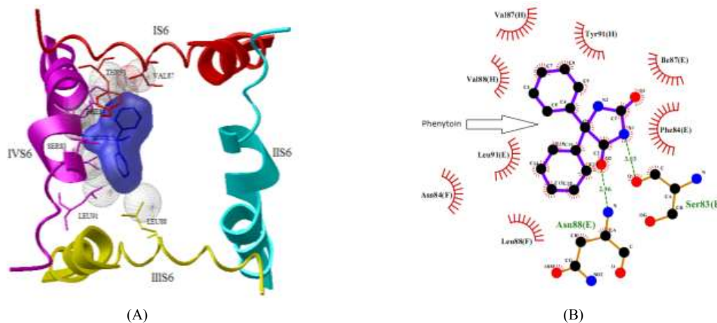
Figure 5. Nav1.2 channel and phenytoin interaction. (a) Cartoon diagram of the channel-drug interactions. (b) Ligplot(18) diagram of the Nav1.2-phenytoin drug interactions. Hydrogen bonds are depicted in green color dotted lines and hydrophobic interaction residues are shown in red color.
